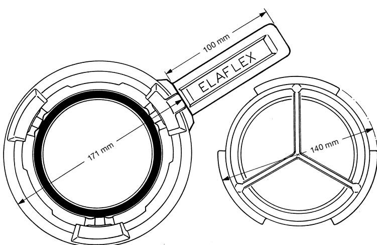
TW- spojka typ MK 100 s tromi tesniacimi lištami TW female coupling MK 100 with 3 locking lugs
